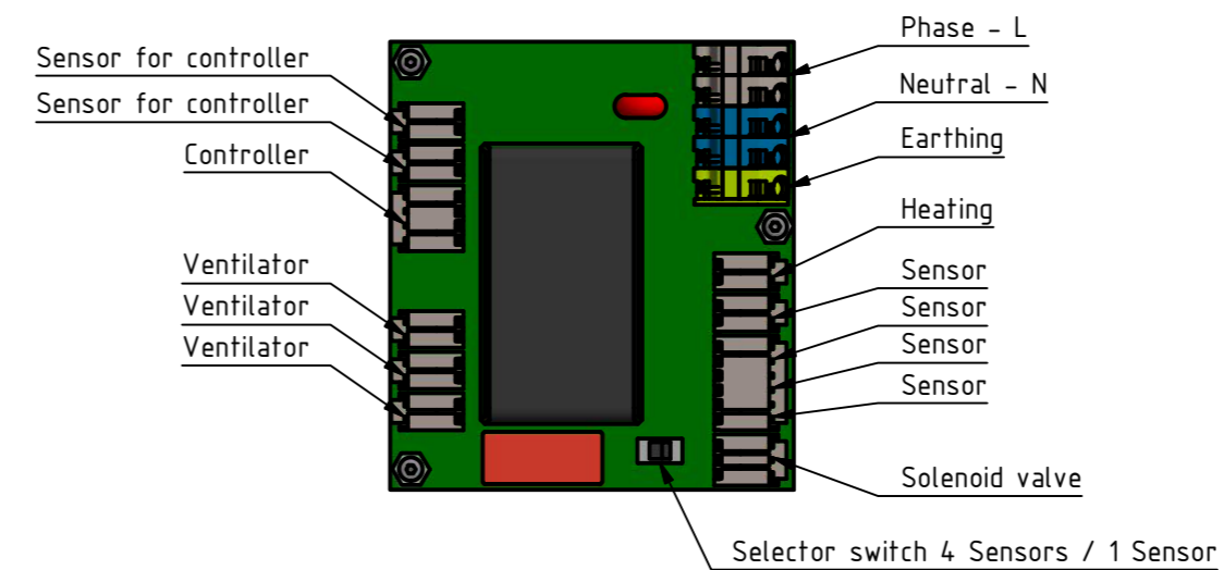
Circuit board ( 1 : 2 )
